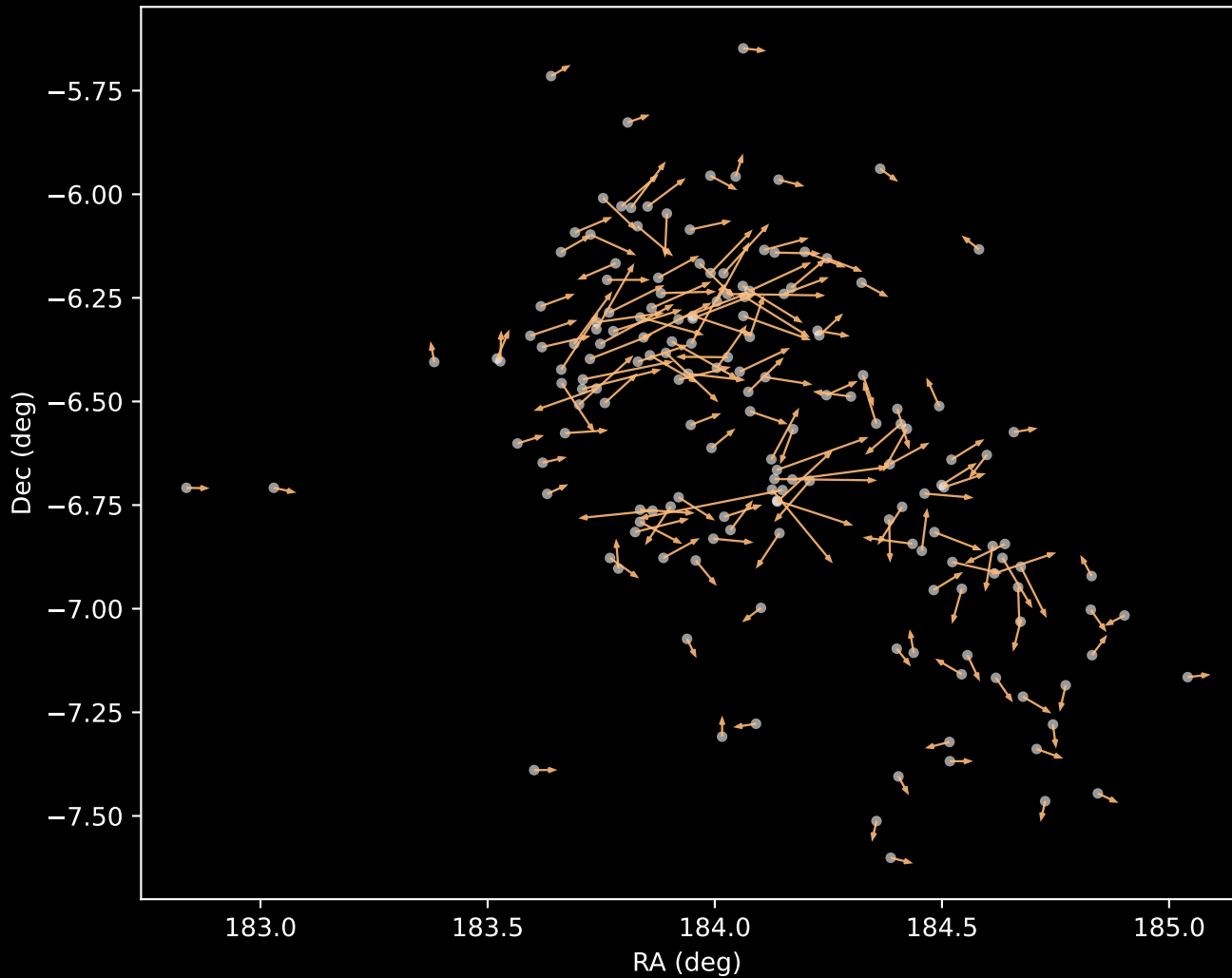
APOGEE DR17 Cluster 3 Proper Motion Vectors (n=168)
