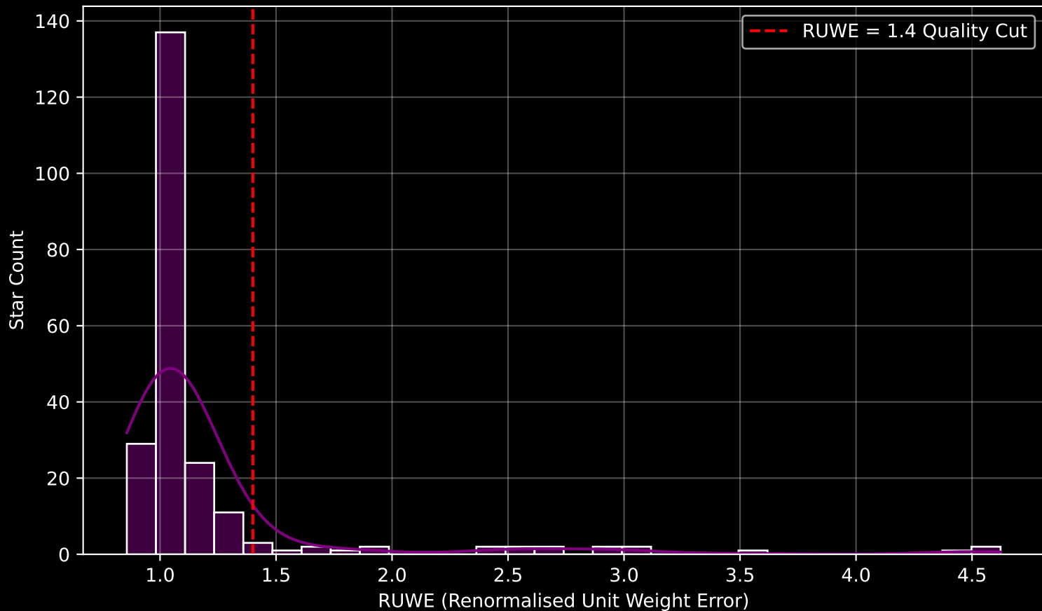
GAPOGEE DR17 Field [ORIONC] RUWE Distribution (n= 224)
