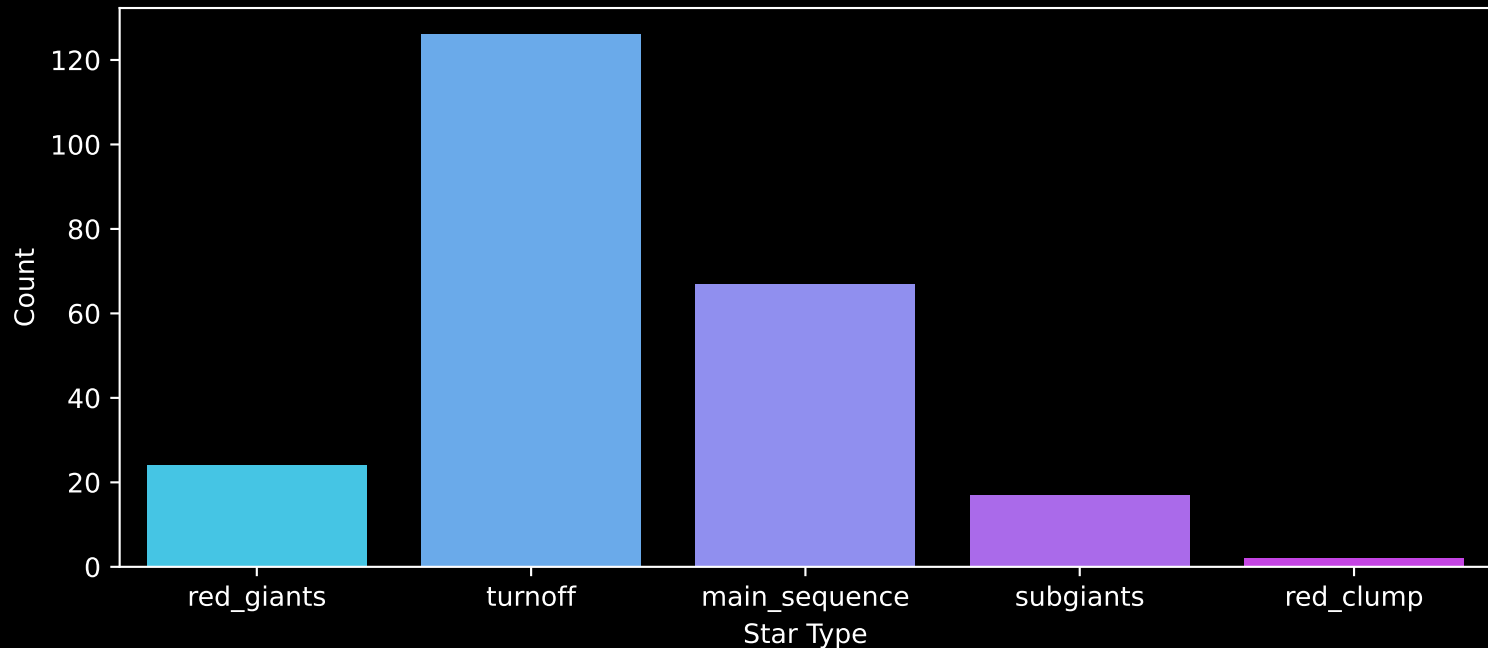
APOGEE DR17 Field: [ORIONC] Count plot of Star Type
