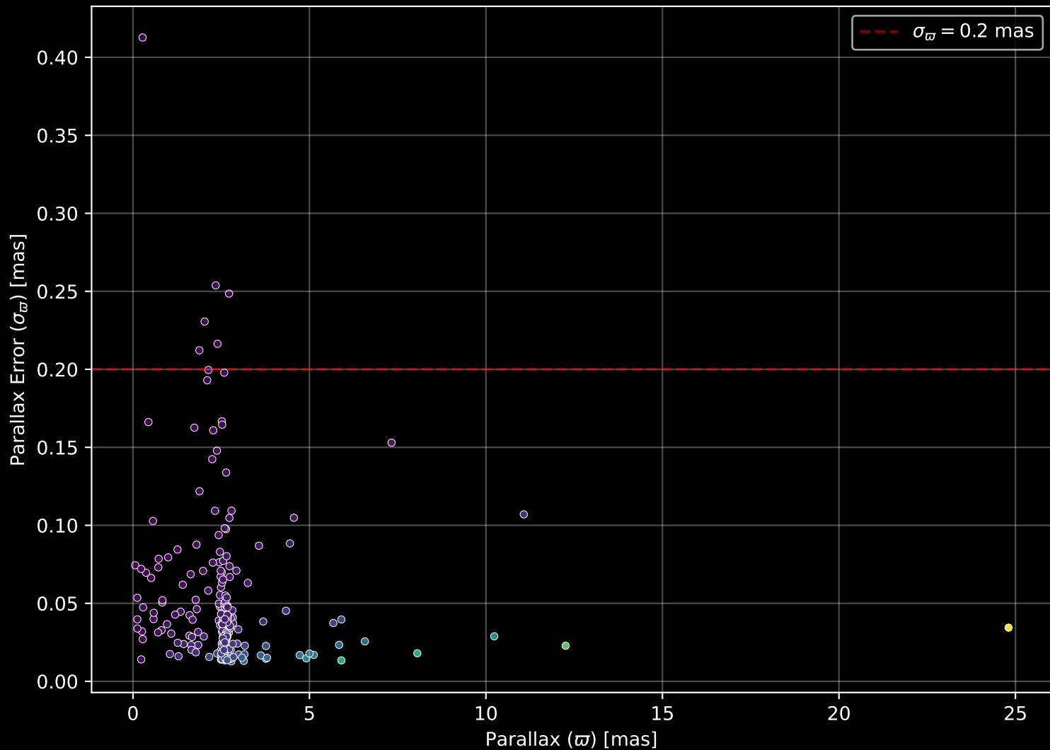
APOGEE DR17 Field: [ORIONC] Parallax Quality (n= 236)
