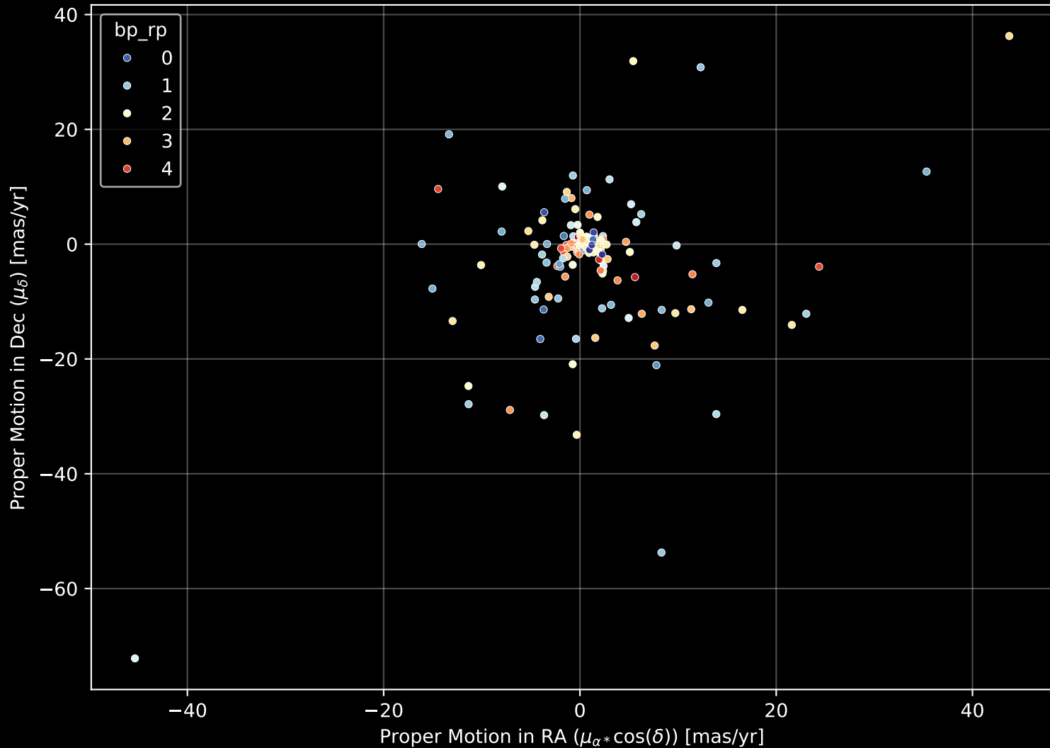
APOGEE DR17 Field: [ORIONC] Proper Motion Diagram (n= 236)
