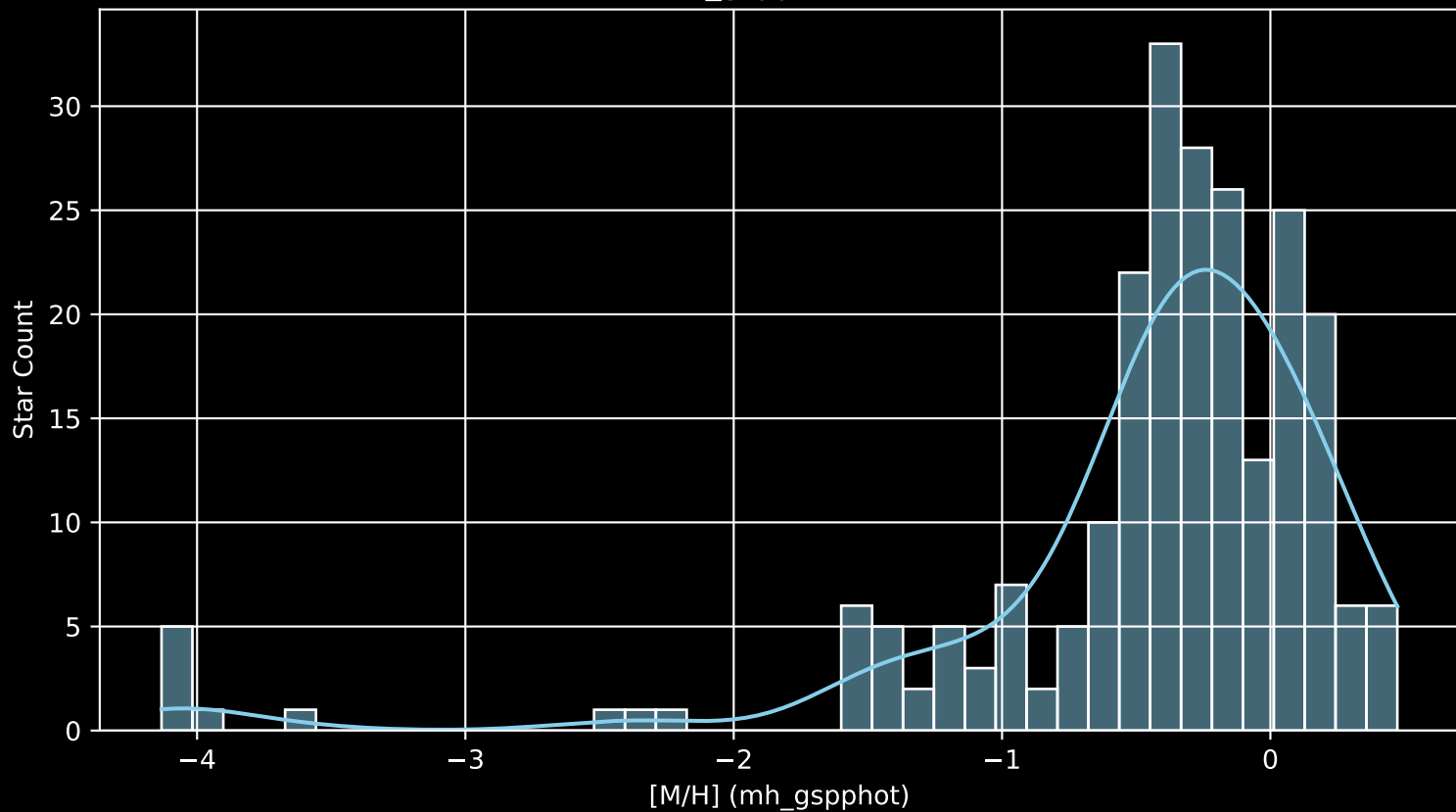
APOGEE DR17 Field: [ORIONC [M/H] (mh_gspphot) (n= 234)
